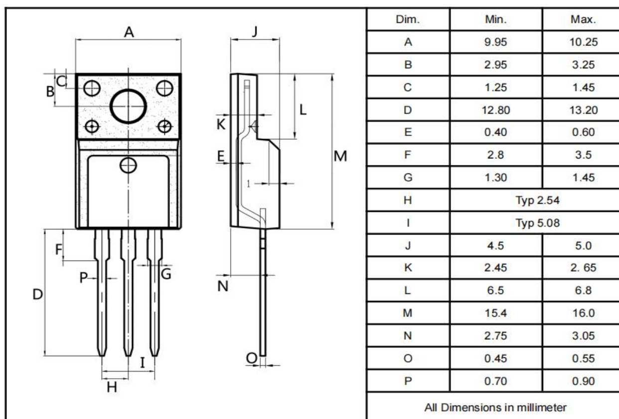
TO-220F
