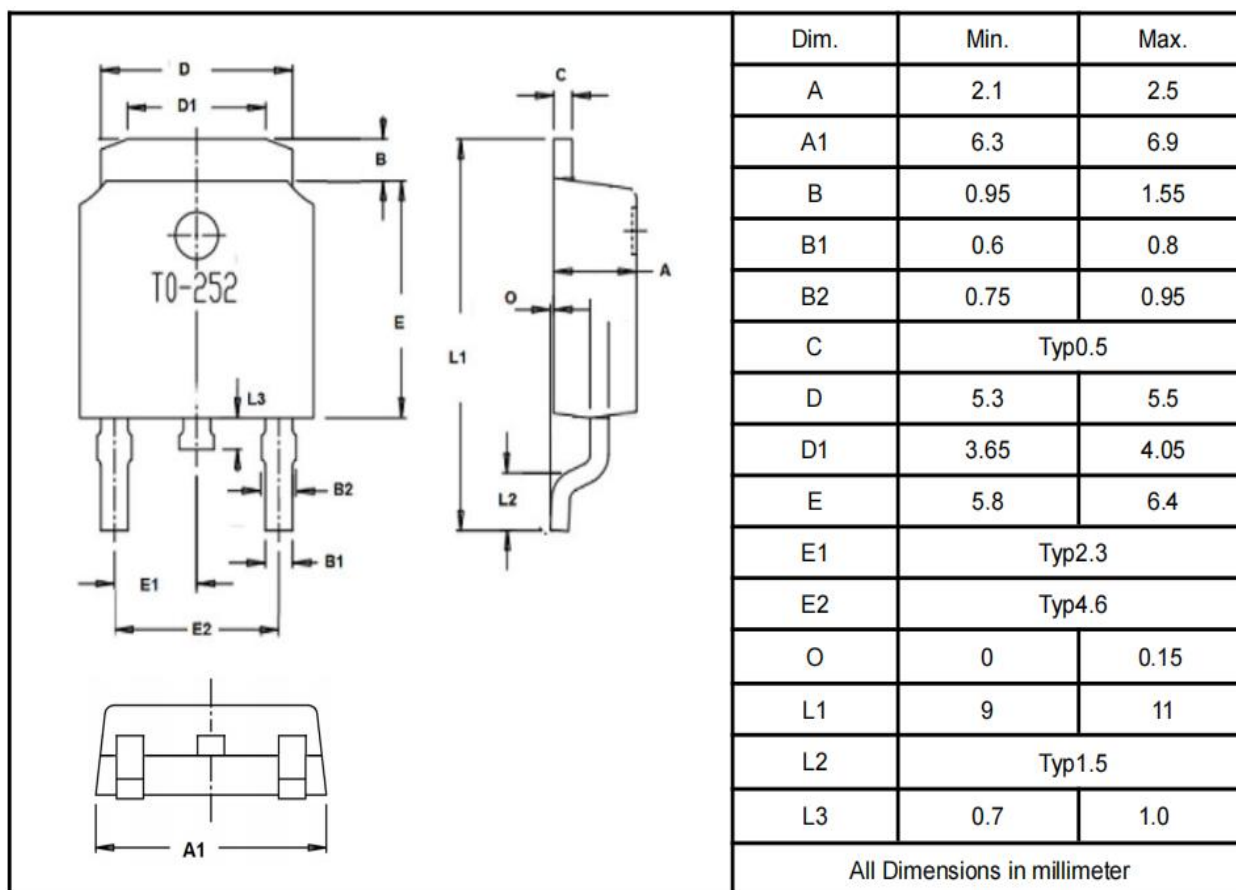
TO-252
